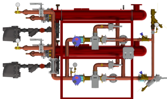
DF8120DWP80-80 Double Wall
